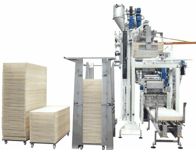
■ Robo XD tray destacker
