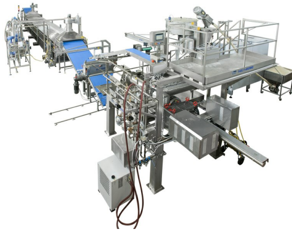
■ Cooker with rods on pre-cooking dough line
